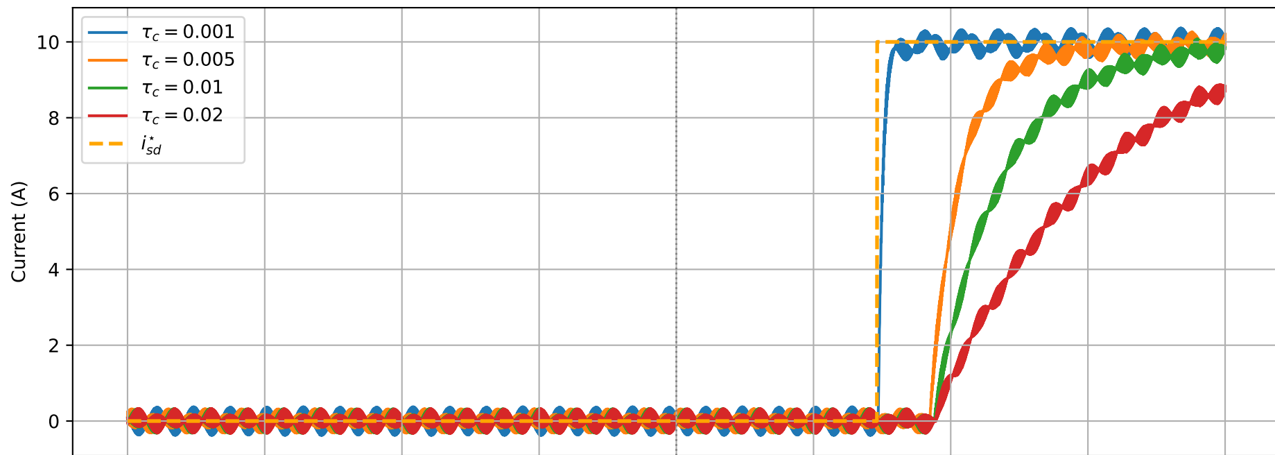
Parametric sweep — \tau_c — zoom at t = 1.5 s
