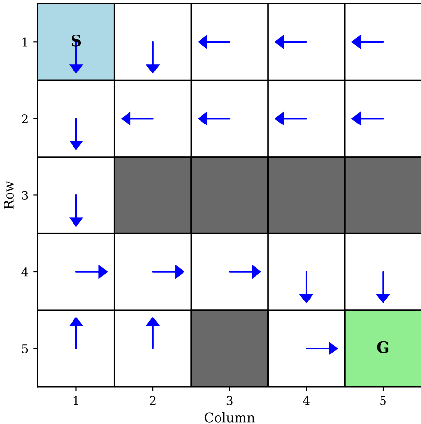
Learned Policy (5×5 HW1 Maze)
