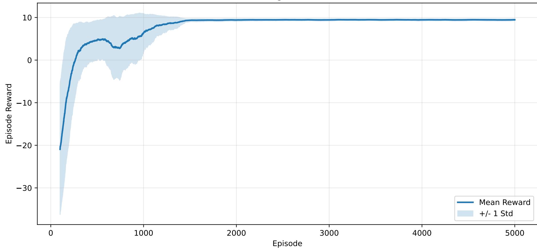
DQN Learning Curves (5 runs)
