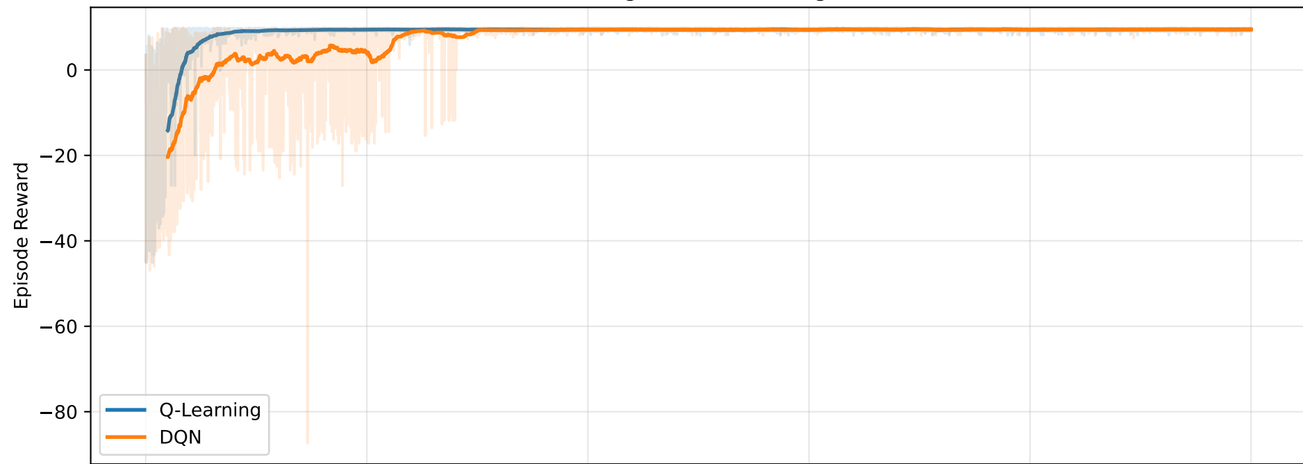
Q-Learning vs DQN Convergence
