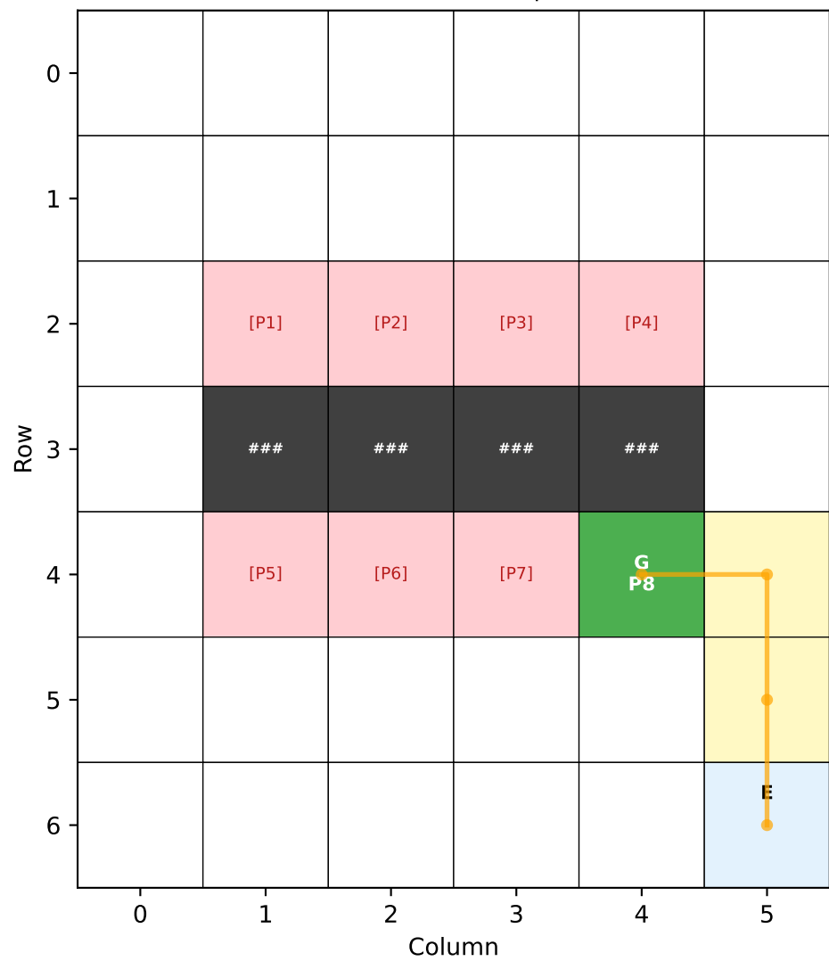
P8 — BFS: 3 steps
