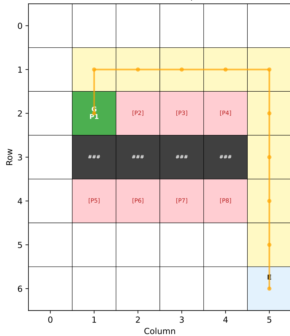
P1 — BFS: 10 steps
