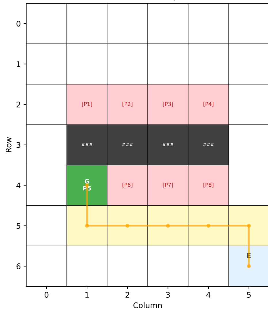
P5 — BFS: 6 steps
