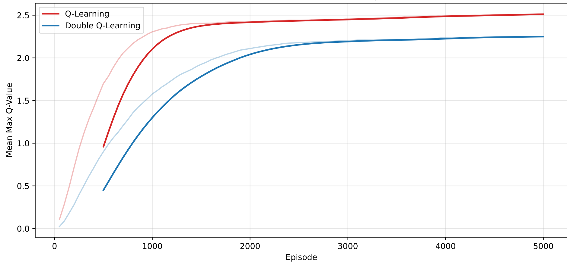
Q-Value Estimates Over Training
