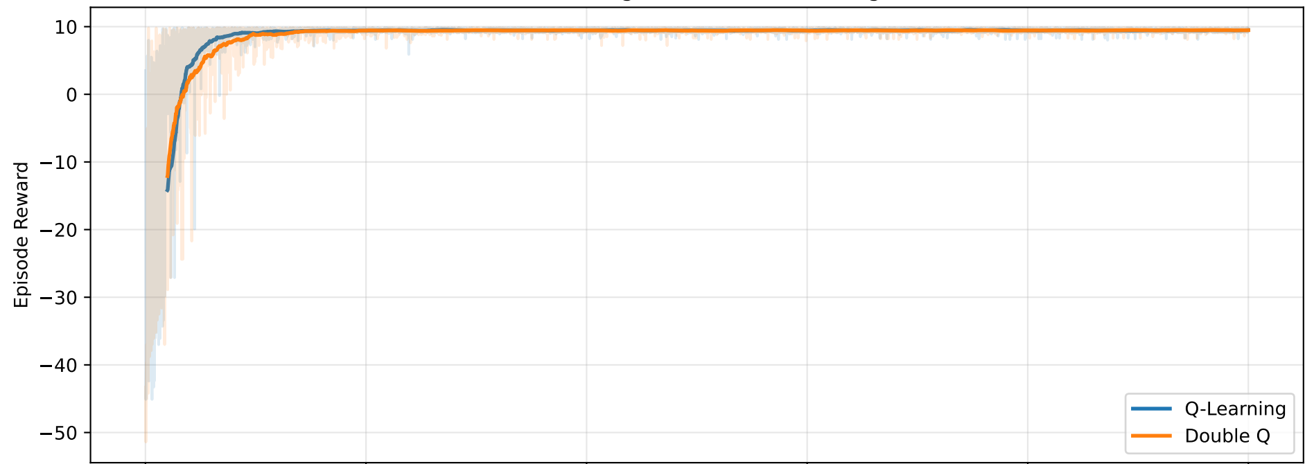
Q-Learning vs Double Q-Learning
