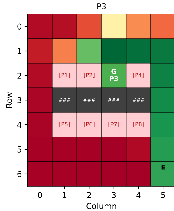
Q-Learning State Values ( V = \max_a Q(s,a) )
