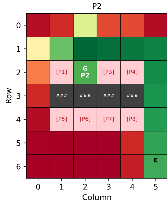
Q-Learning State Values ( V = \max_a Q(s,a) )
