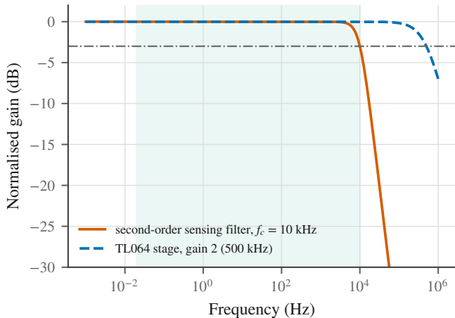
(b) Sensing filter and drive stage
