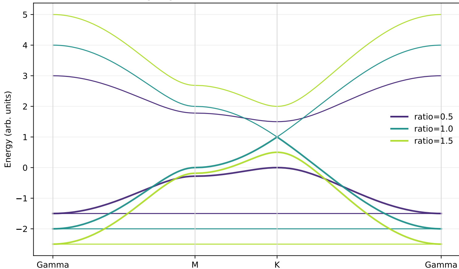
Breathing Kagome Bands: Gamma-M-K-Gamma (overlaid)
