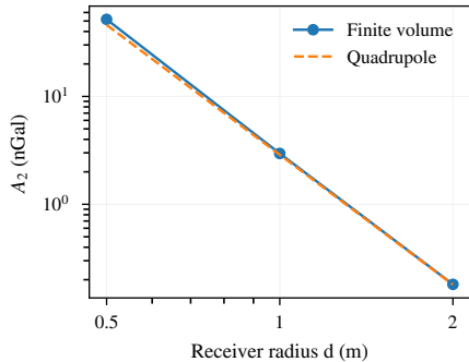
(c) Distance dependence
