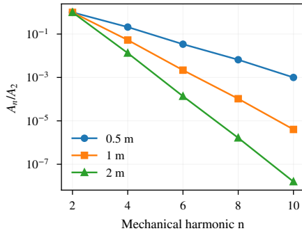
(b) Harmonic content
