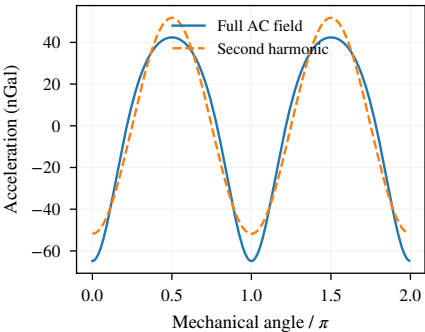
(a) Waveform at d = 0.5 m
