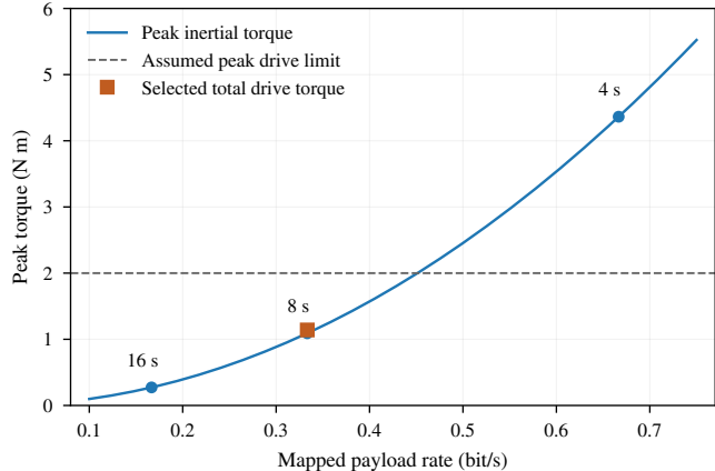
(b) Seven-tone CF-FSK mechanical demand
