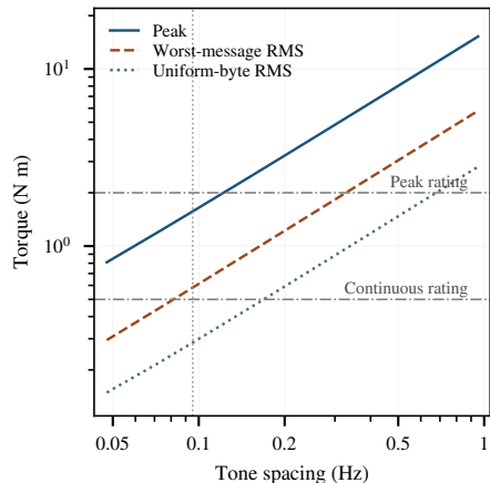
(c) Drive: same waveforms
