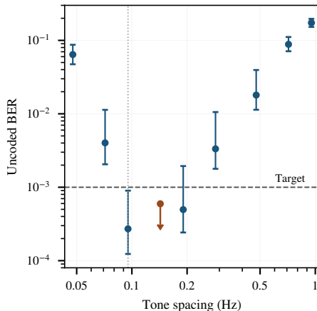
(b) Receiver: 1.75 s symbols
