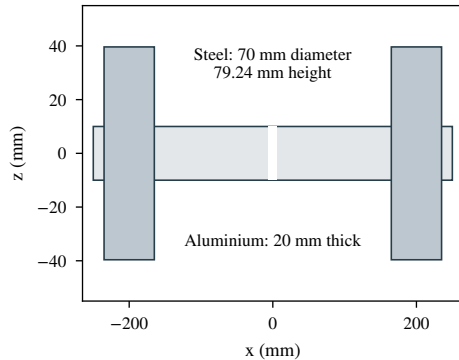
(b) Axial section, y = 0
