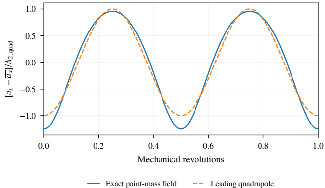
(b) Two signal cycles per revolution ( d/r=3 )
