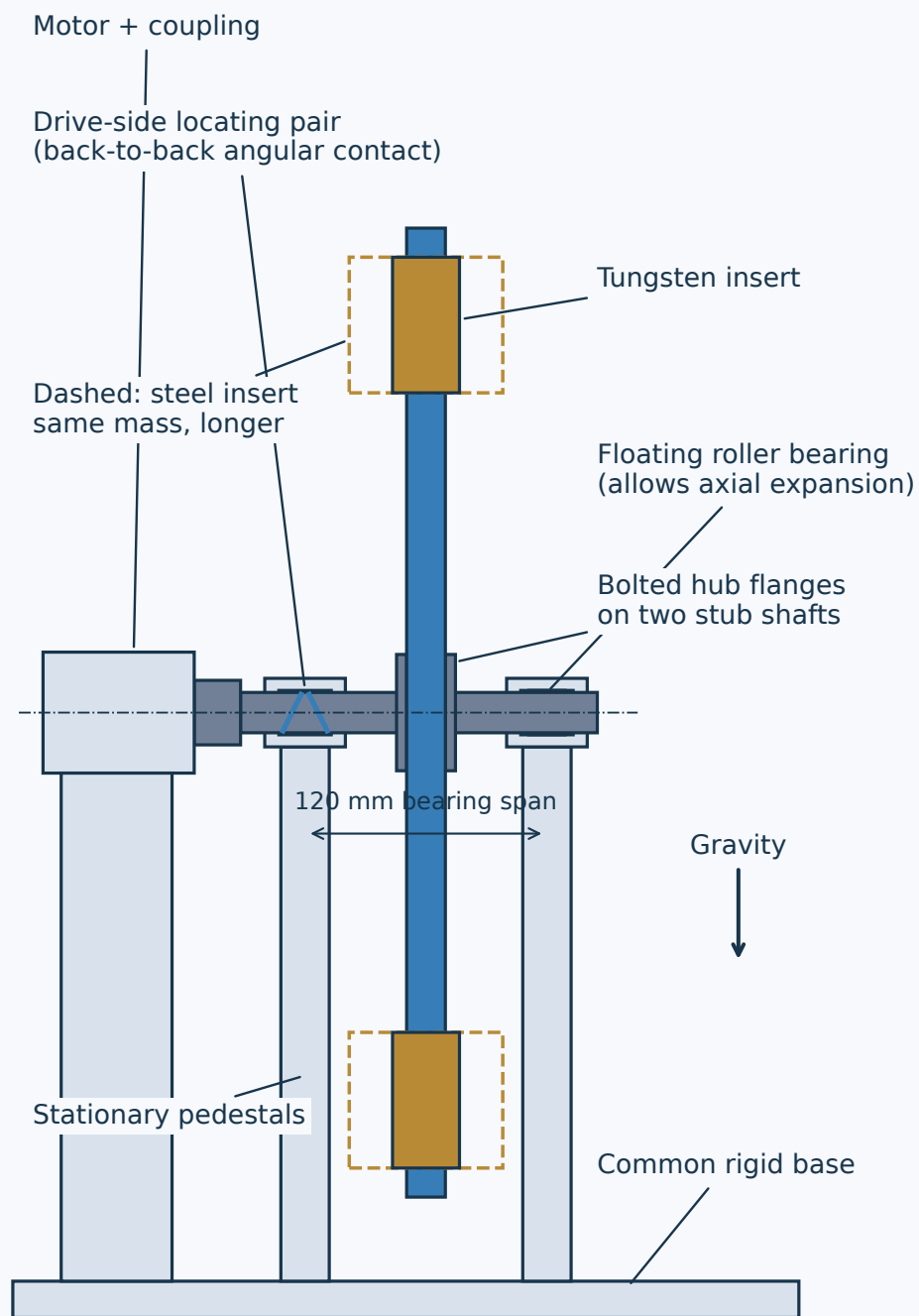
B Edge view of the rotor Horizontal shaft supported on both sides
