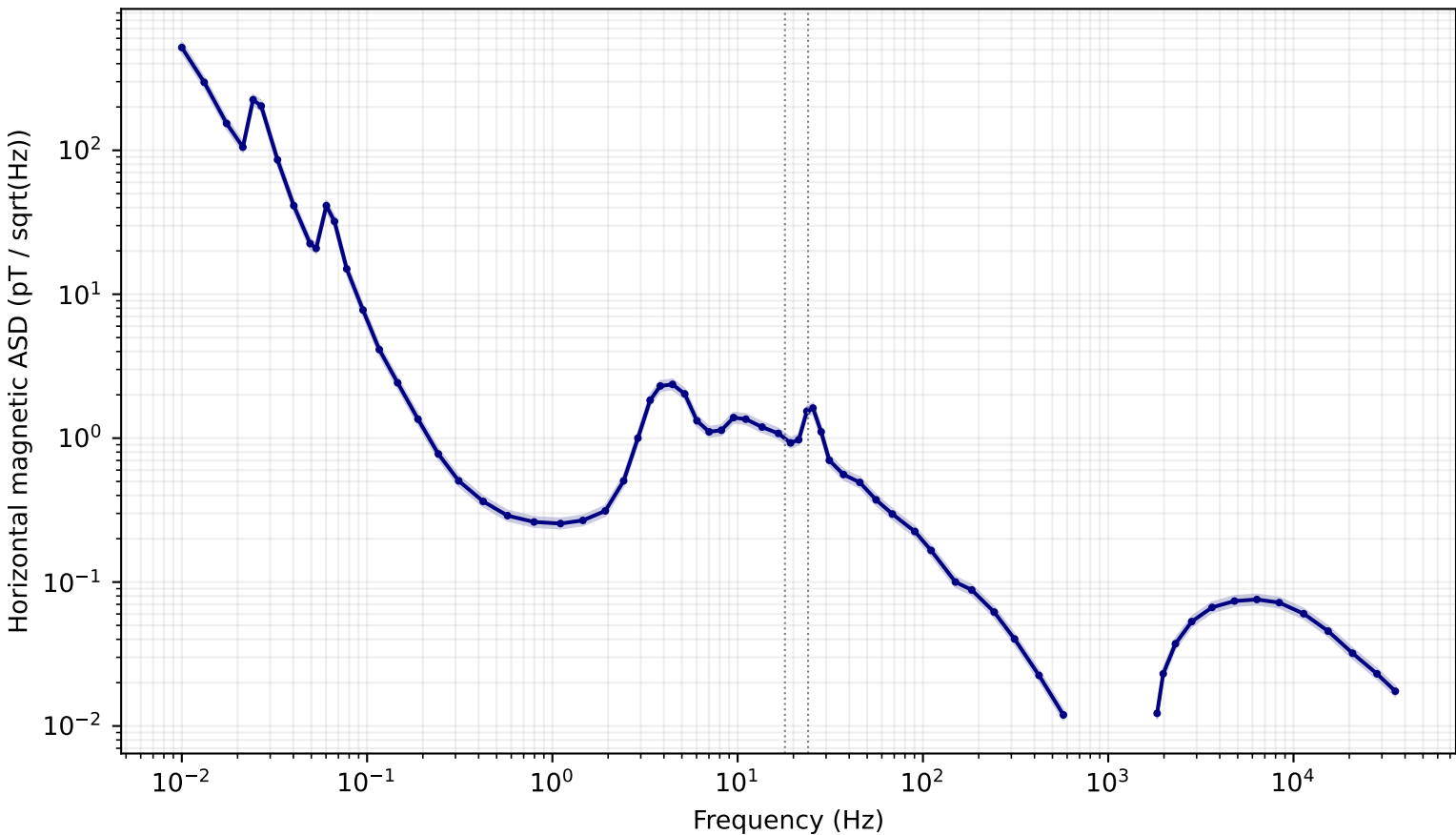
Macnae historical nominal background: digitized broadband trace
