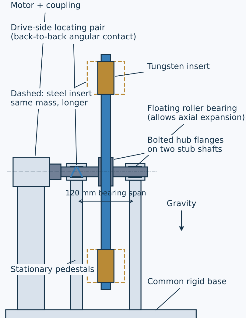
B Edge view of the rotor Horizontal shaft supported on both sides
