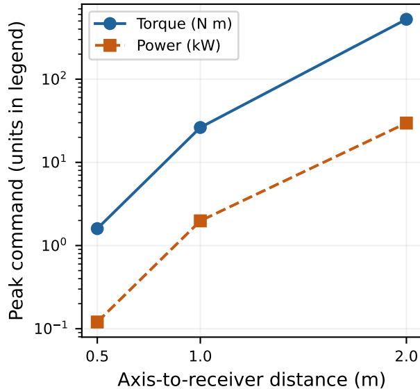
(b) Inertial drive demand
