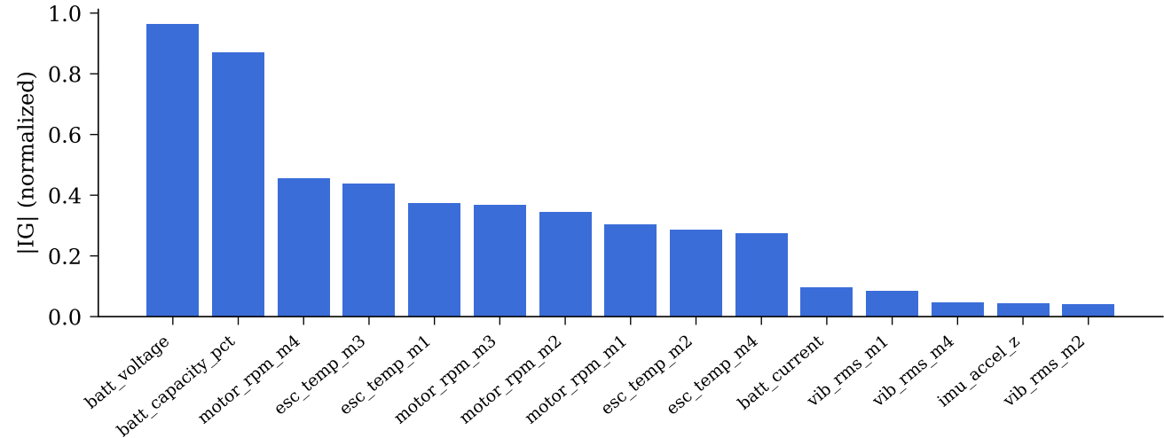
Mean sensor attribution across UAV assets
