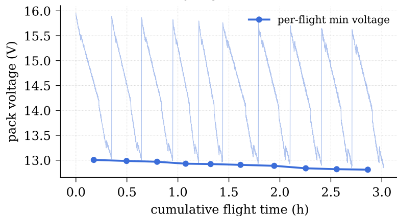
(c) Battery degradation · UAV-000
