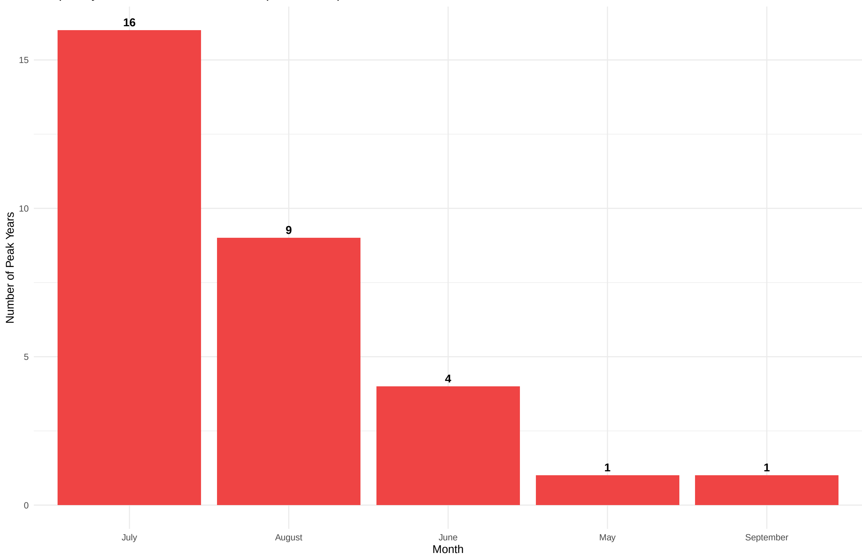
Frequency of Heatwave Peak Months (1990–2024)
