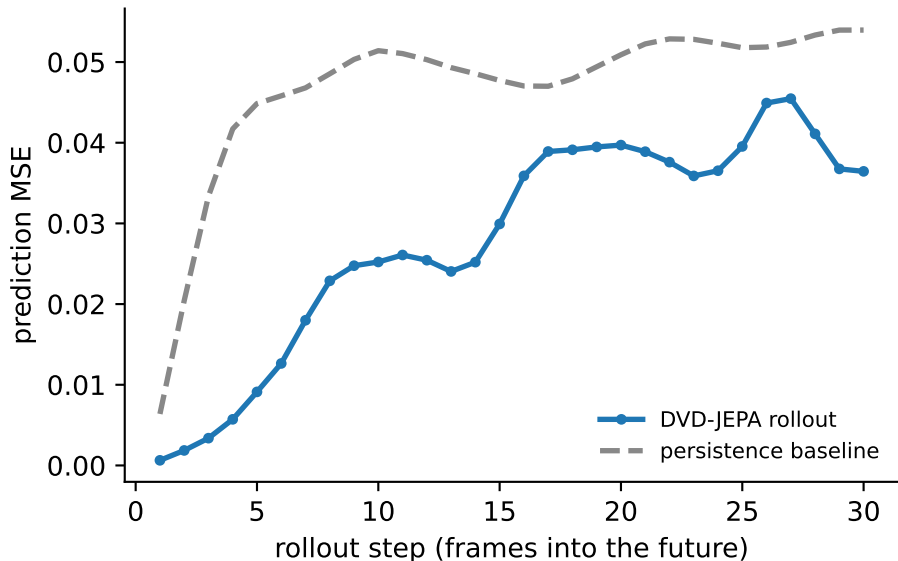
Latent rollout tracks the future, then drifts
