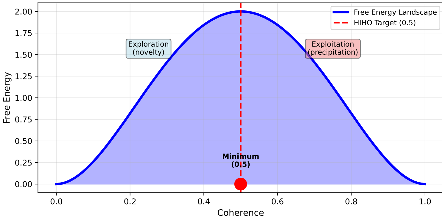
FIG. 5: HIHO Double-Well Potential
