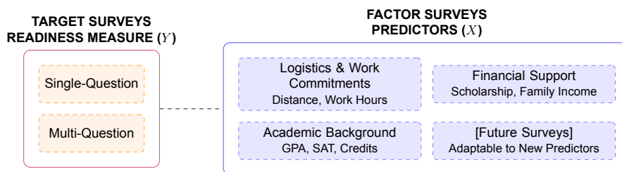
Figure 2: Dual-Survey Architecture. Target Surveys collect the readiness measure ( Y ), and Factor Surveys collect predictors ( X ). Dashed lines show linkage relationships that enable flexible study configurations.
