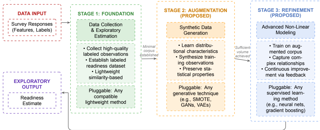
Figure 4: The Three-Stage Progressive Pipeline. Each stage represents a pluggable component that can be substituted with alternative algorithms. The framework progresses from data acquisition through augmentation to refined prediction. The survey workflow, readiness calculation, and exploratory model path are foundation components; augmentation and refinement remain future work.
