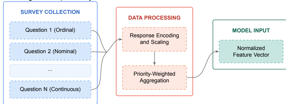
Figure 3: Survey data processing pipeline. Raw responses undergo type-aware encoding and scaling followed by priority-weighted aggregation to produce standardized feature vectors for readiness scoring and exploratory model evaluation.
