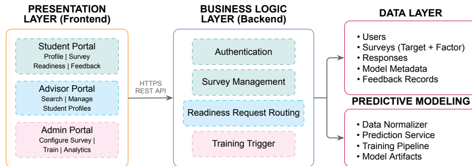
Figure 1: ACOSUS system architecture. Four layers separate presentation, business logic, data persistence, and predictive modeling, enabling independent scaling and clear separation of responsibilities.
