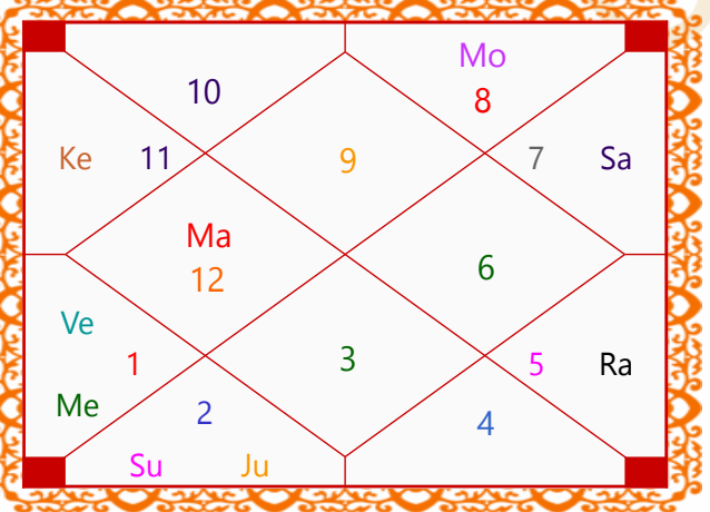
Dasamamsa Chart
