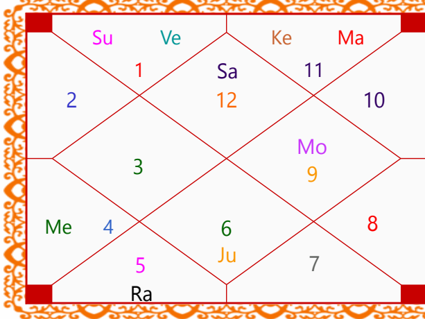
Dreshkana Chart
