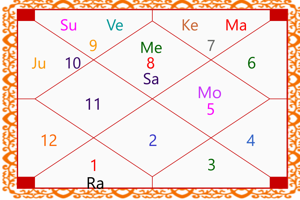
Lagna Chart
