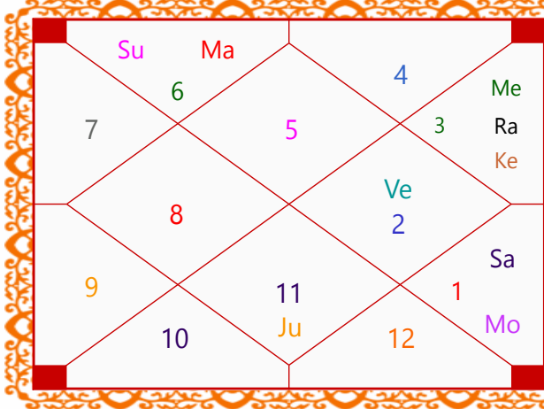
Chaturvimsamsa Chart
