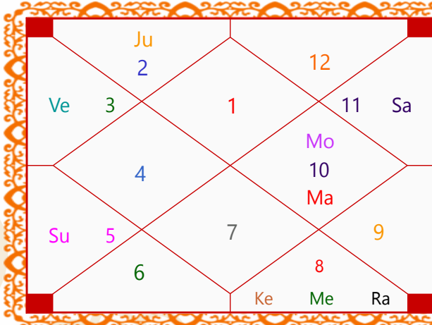
Shodasamsa Chart
