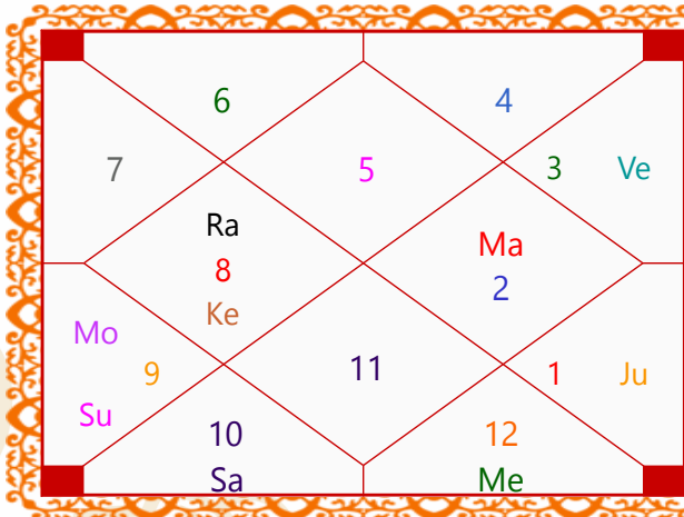
Akshavedamsa Chart
