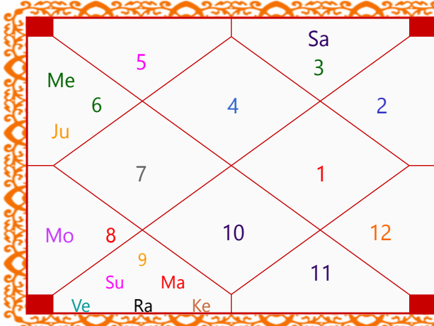
Panchamsa Chart
