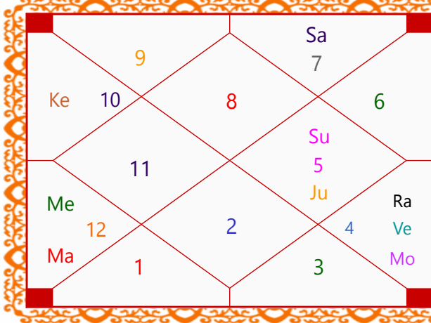
Navamsa Chart
