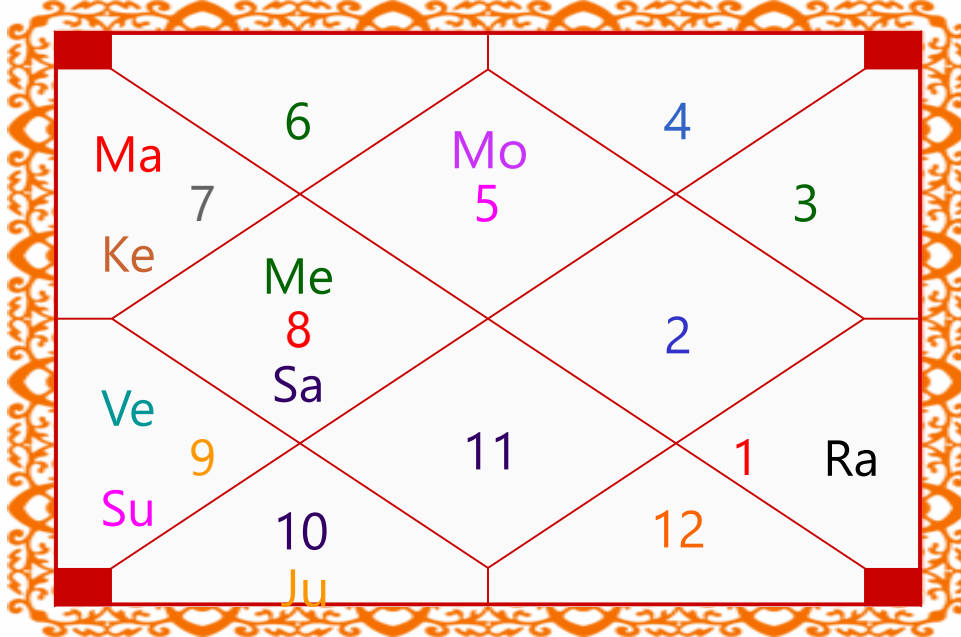
Moon Chart
