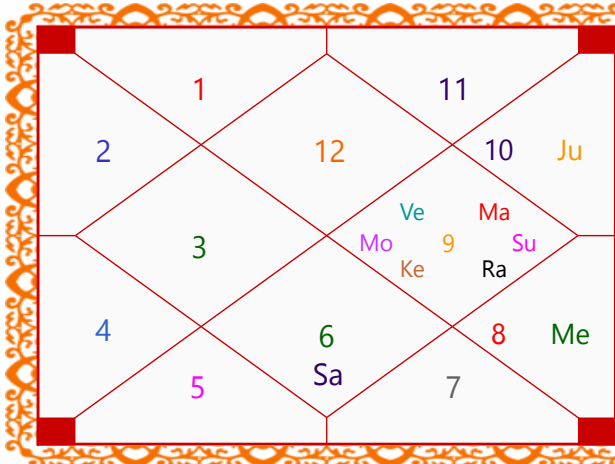
Trimsamsa Chart
