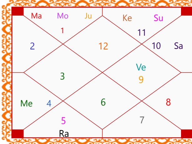
Ekadasamsa Chart
