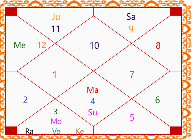
Shastamsa Chart
