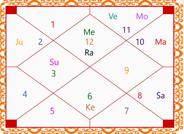
Saptavimsamsa Chart
