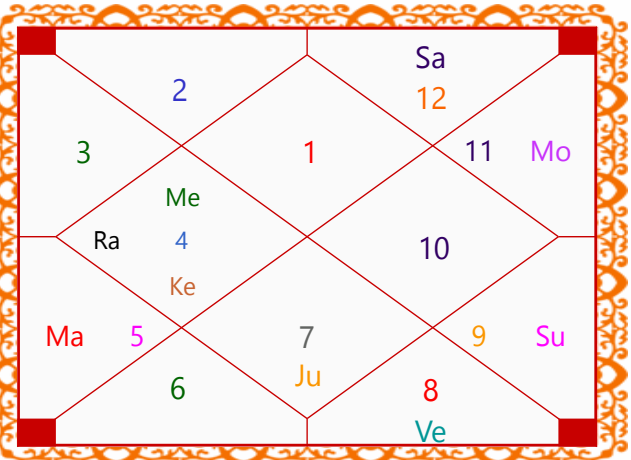
Ashtamsa Chart
