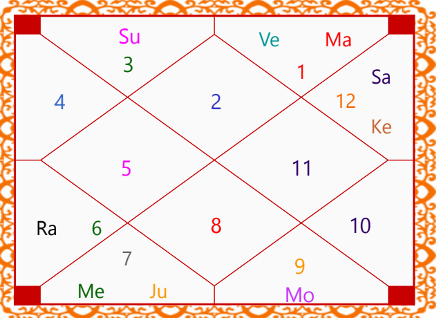
Dwadasamsa Chart
