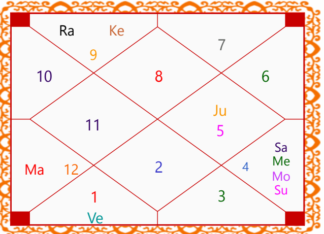
Vimsamsa Chart
