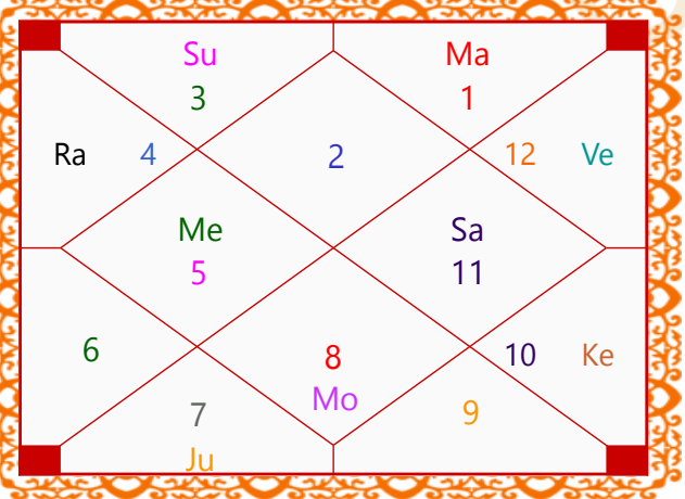
Chaturthamsa Chart
