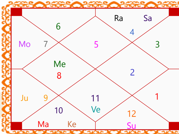
Saptamamsa Chart
