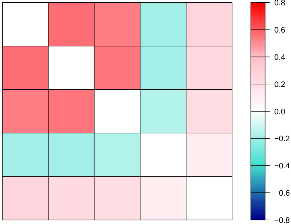
True Mean of FC
