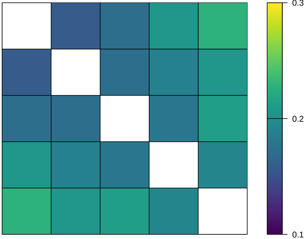
True SD of FC
