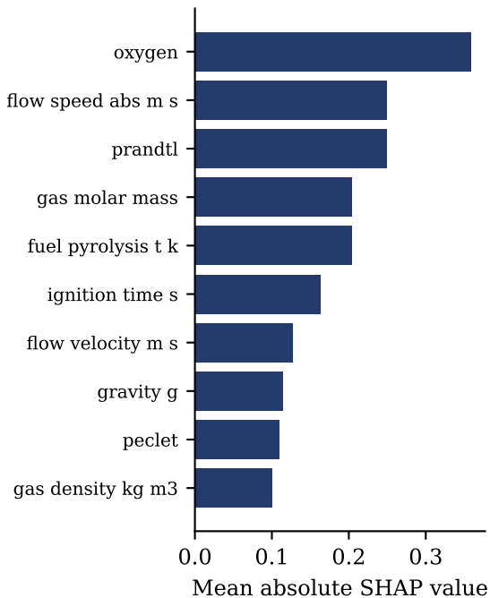
Ignition classifier
