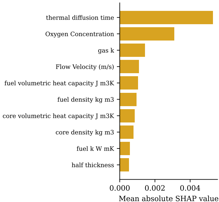
FSR regressor
