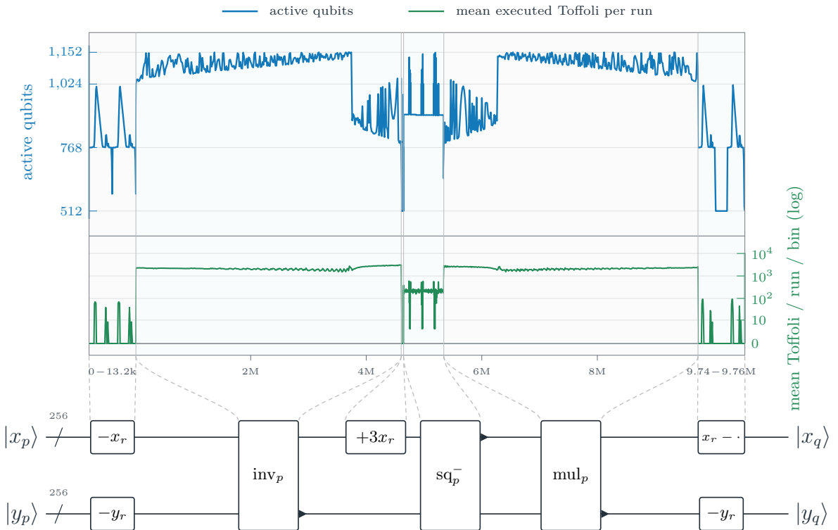
Fig. 1: Active-qubit liveness and mean executed Toffoli gates per run across six circuit phases. Toffoli counts include CCX + CCZ and use a logarithmic axis. The initial and final subtraction phases use separate compressed horizontal scales; the four central phases share one operation-index scale.
