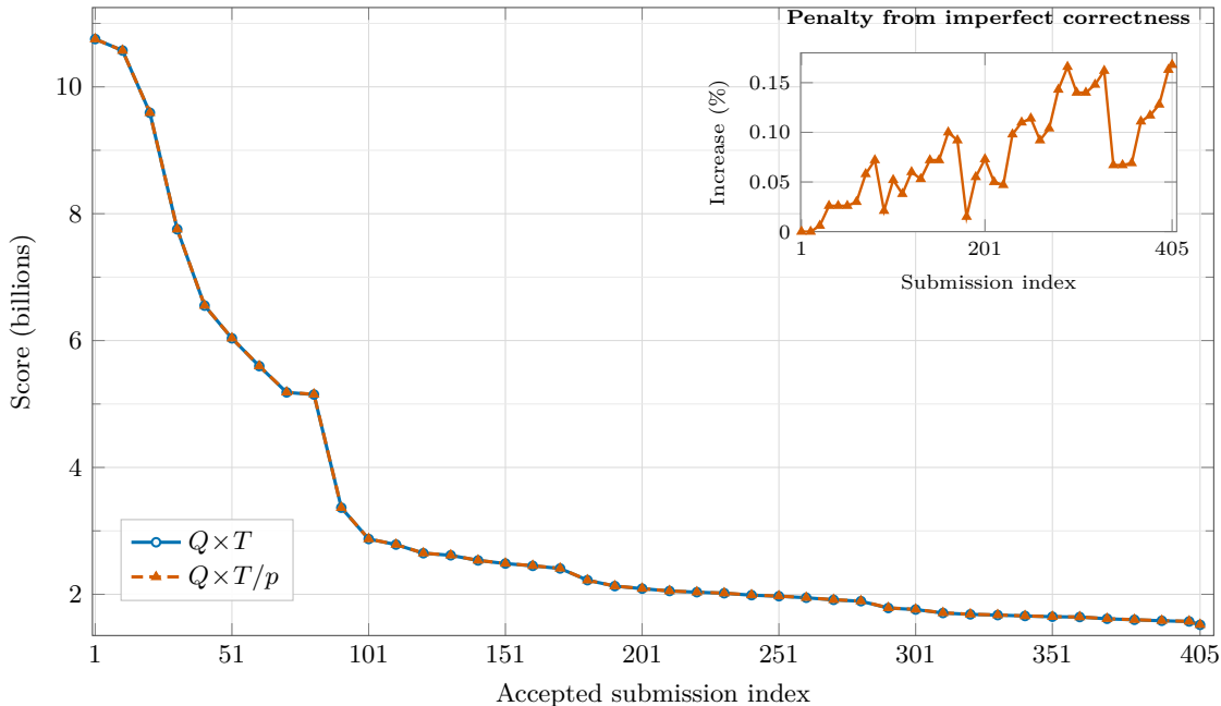
Historical circuit score on 50,000 fixed point pairs
