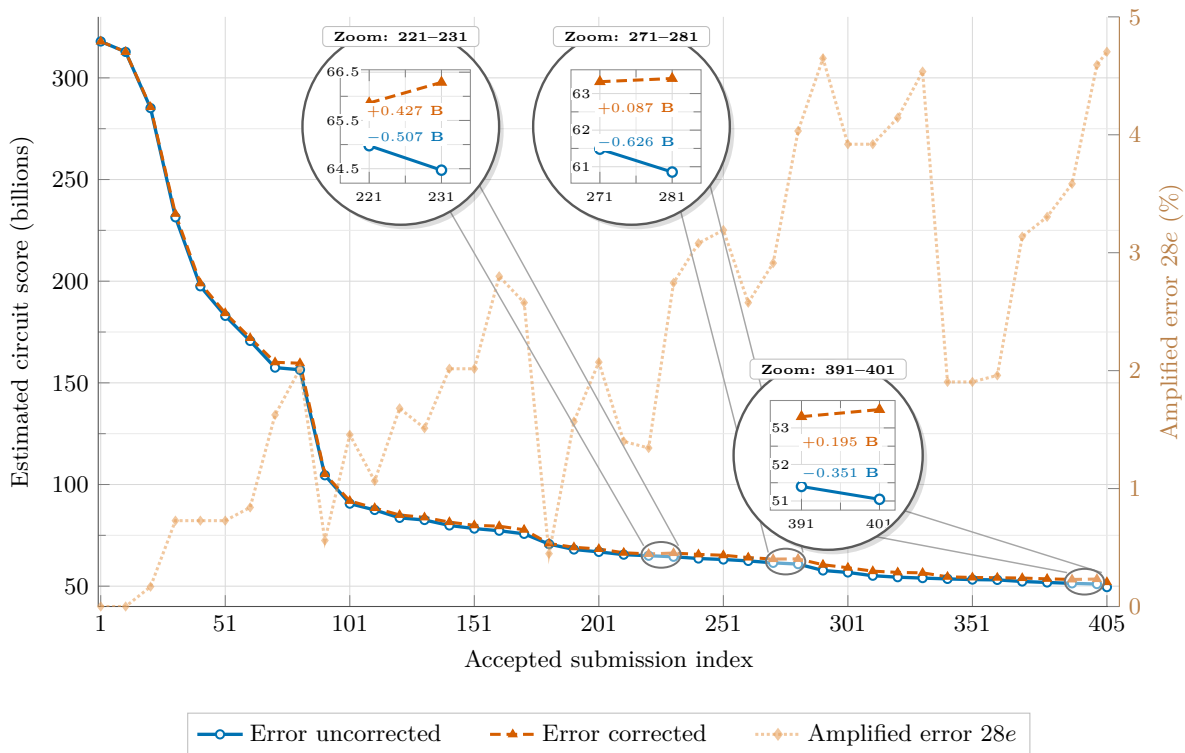
Estimated full Shor circuit cost for 28 point additions
