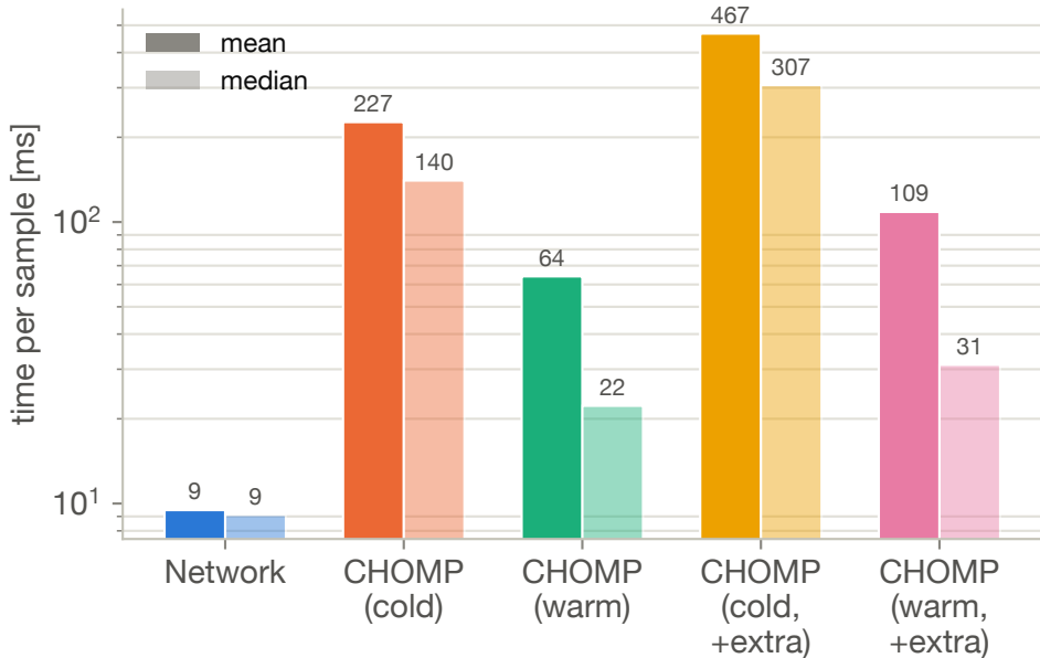
Computation time (N = 100 samples)
