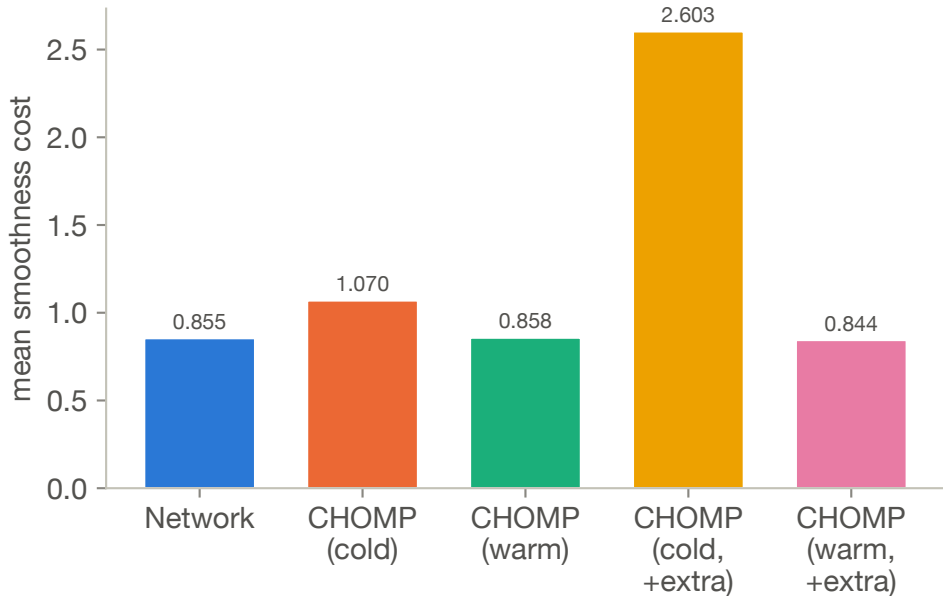
Smoothness (lower = smoother) (N = 100 samples)
