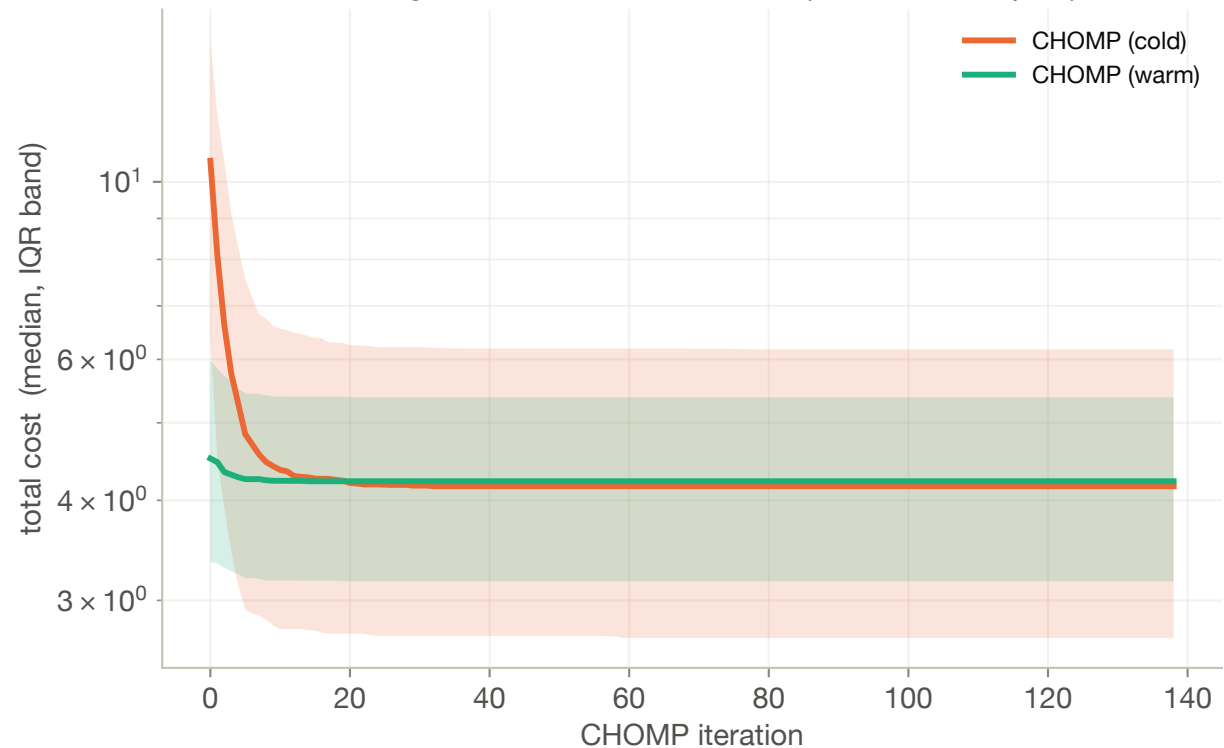
Convergence: warm vs. cold start (N = 1000 samples)
