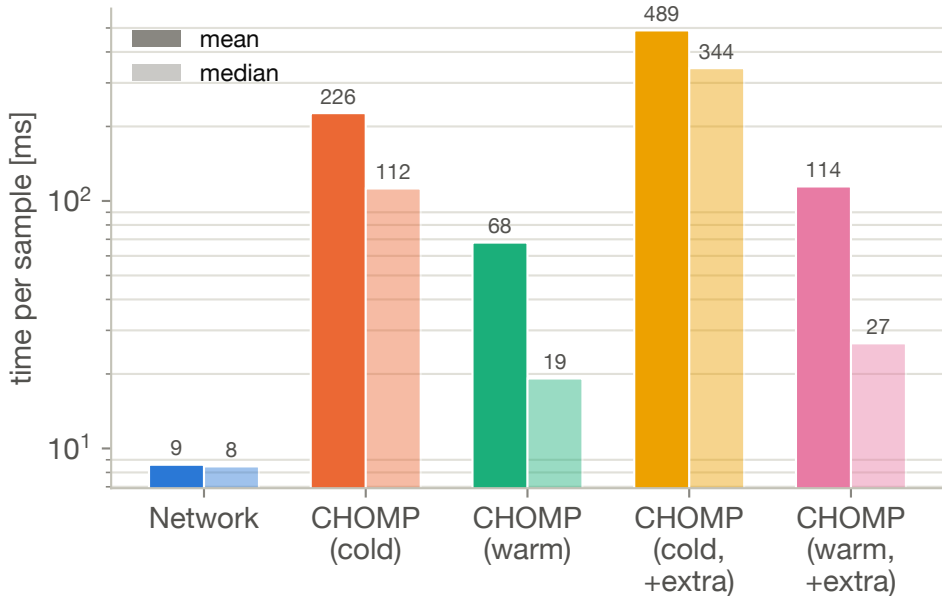
Computation time (N = 1000 samples)
