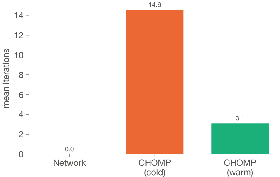
Iterations to convergence (N = 1000 samples)
