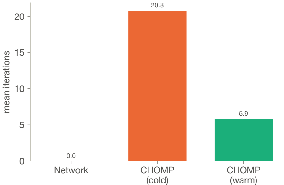
Iterations to convergence (N = 1000 samples)
