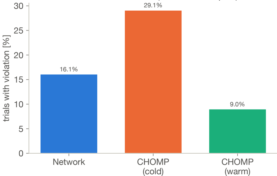
Joint-limit violations (N = 1000 samples)
