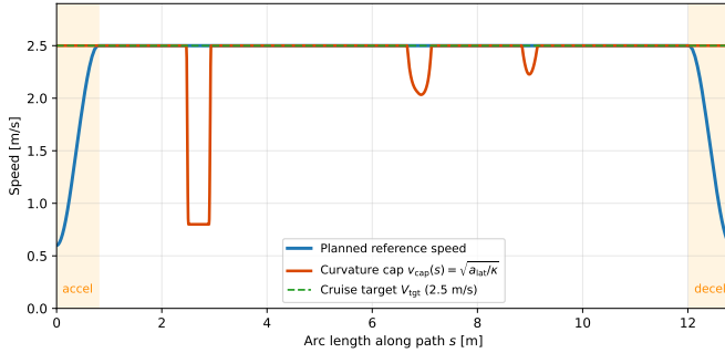
Fig. 4. Speed along the planned path: the planner cruises at the target V_{\text{tgt}} (trapezoidal, with accel/decel ramps), while the controller’s curvature cap v_{\text{cap}}(s) = \sqrt{a_{\text{lat}}^{\text{max}}/\kappa(s)} lowers the effective target into corners (down to the floor v_{\text{min}} ) and leaves straights at full speed.
