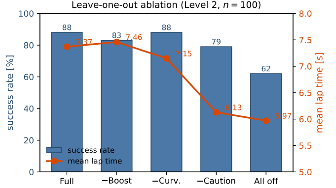
Fig. 5. Leave-one-out ablation on Level 2 ( n = 100 ): success rate (bars, left) and mean lap time (line, right). Caution is the dominant robustness lever; removing all rules yields the fast but fragile raw MPCC.
