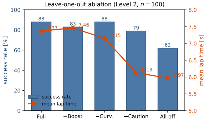
Fig. 5. Leave-one-out ablation on Level 2 ( n = 100 ): success rate (bars, left) and mean lap time (line, right). Caution is the dominant robustness lever; removing all rules yields the fast but fragile raw MPCC.
