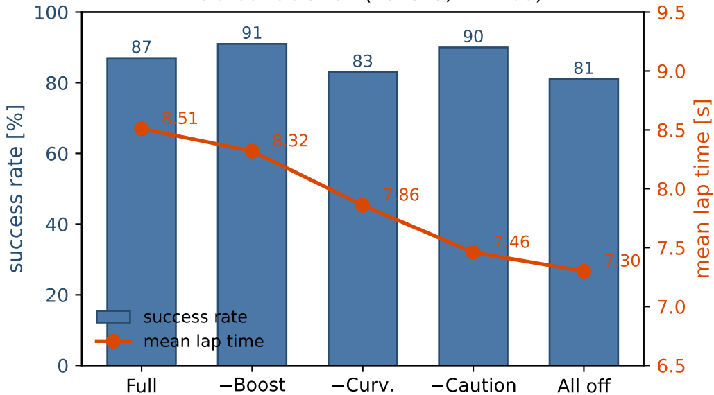
Held-out ablation (Level 3, n = 100 )
