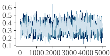
pi_10
