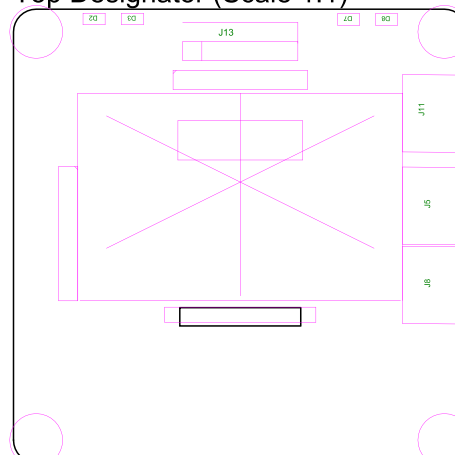
Top Designator (Scale 1:1)
