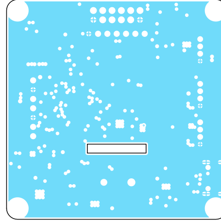
Int2 (GND) (Scale 1:1)
