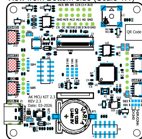
View from Bottom side (Scale 1:1)
