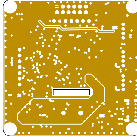
Int1 (PWR) (Scale 1:1)
