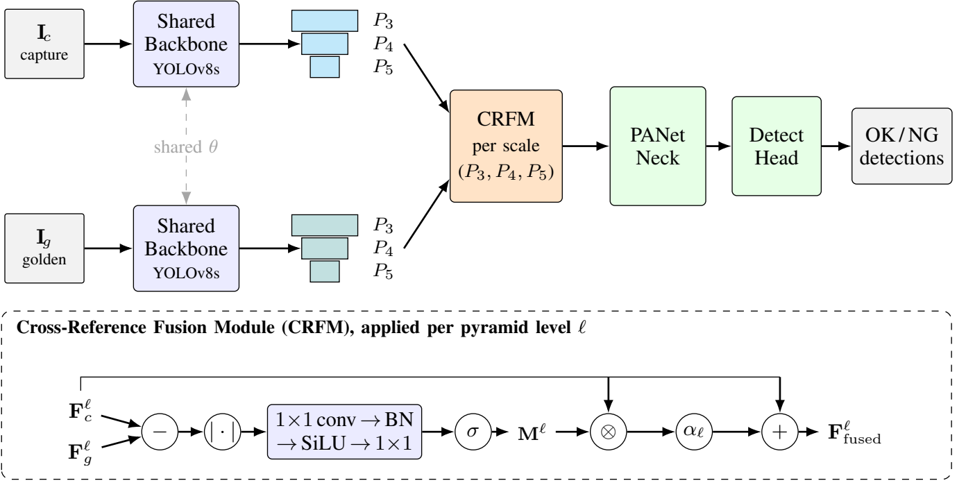
Fig. 1. Architecture of the proposed Dual-Stream YOLO (DS-YOLO). The captured frame I_c and the always-available golden reference I_g (pre-registered by the fixed camera and fixture) are encoded by a shared (Siamese) YOLOv8s backbone. At every pyramid level \ell \in \{P_3, P_4, P_5\} a Cross-Reference Fusion Module (CRFM) fuses the capture and golden features through a learnable difference-attention gate (inset): M^\ell = \sigma(g_\ell(|F_c^\ell - F_g^\ell|)) and F_{\text{fused}}^\ell = F_c^\ell + \alpha_\ell M^\ell \odot F_g^\ell , with \alpha_\ell initialised to 0 so the network starts exactly as the YOLOv8s baseline. The fused feature pyramid feeds the unmodified PANet neck and Detect head, which output per-component OK/NG detections.
