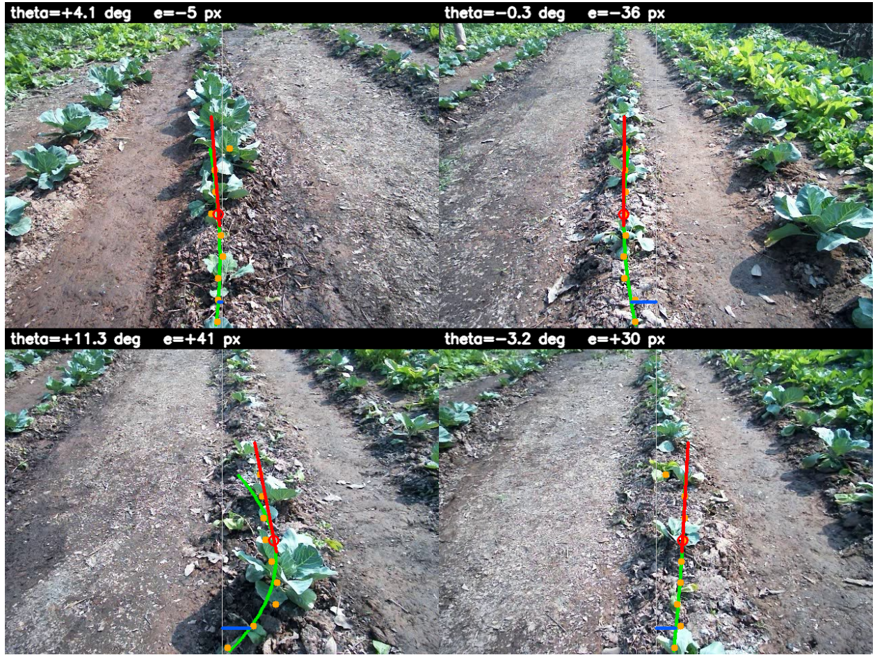
Figure 5: Qualitative behaviour of the detector-free estimator on four real forward-view cabbage frames spanning a range of canopy density (each panel overlays the Excess-Green column-peak track in orange, the robust quadratic guidance curve x = P(y) in green, the look-ahead tangent/heading in red, and the near-row cross-track in blue; the reported \theta and e are printed). The tracker follows the central cabbage row from densely planted rows through sparse, gapped stretches to young transplants. These panels are illustrative, not a correctness measurement (cf. Section 4.4).
