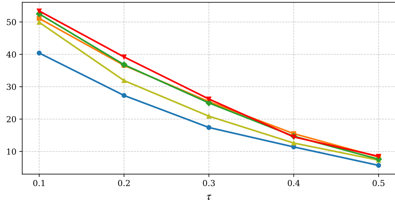
GPQA
