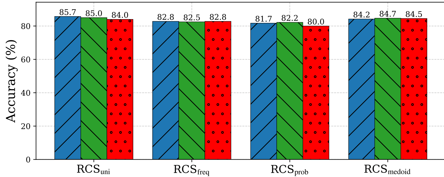
Arithmetics
