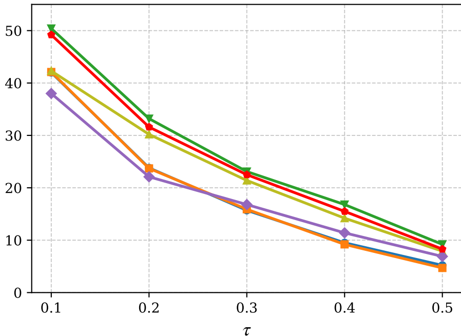
GPQA
