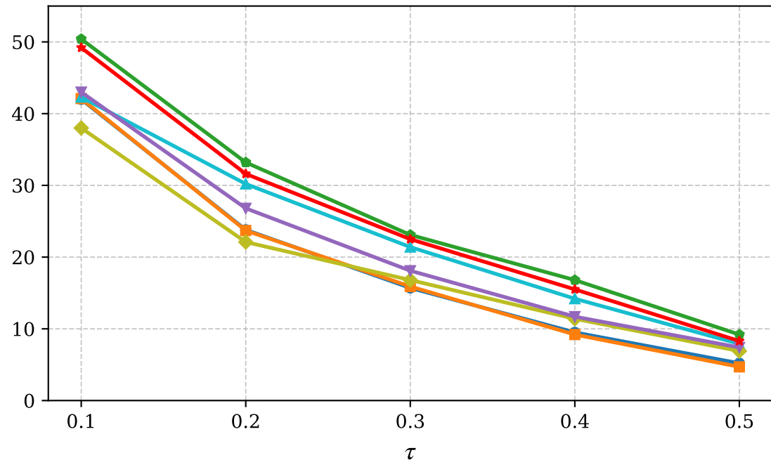
GPQA
