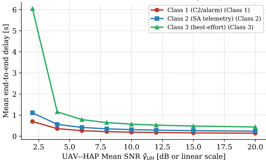
Class-wise end-to-end mean delay vs. \bar{\gamma}_{UH}
